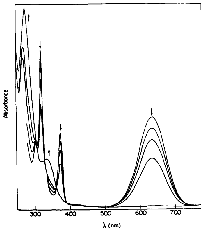
Fig. 3. Spectral changes upon irradiation of [\text{Ir}_2(\text{TMB})_4](\text{B}(\text{C}_6\text{H}_5)_4)_2 in neat 1,2-dichloroethane ( \lambda_{\text{ex}} > 604 \text{ nm} ).
