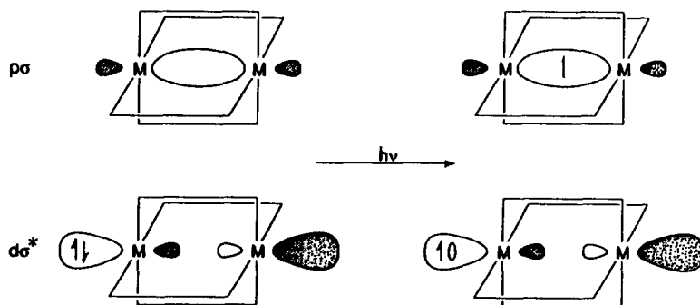
Fig. 1. Pictorial representation of the M_2 -localized hole in the ^3(d\sigma^* p\sigma) state of a face-to-face binuclear d^8 complex. Prototypal complexes are Rh_2b_4^{2+} ( b = 1,3 -diisocyanopropane), Rh_2(TMB)_4^{2+} ( TMB = 2,5 -diisocyno-2,5-dimethylhexane), Ir_2(TMB)_4^{2+} , and Pt_2(P_2O_5H_2)_4^{4-} . Similar orbitals describe the lowest excited states of [Ir(\mu\text{-}pz)COD]_2 ( pz = pyrazole; COD = 1,5 -cyclooctadiene).
